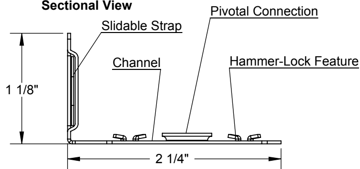
Sectional View
