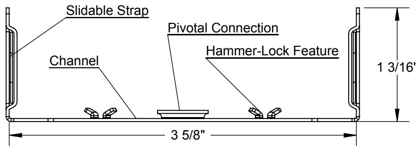
Sectional View
