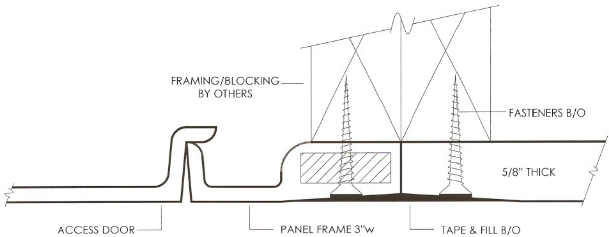
TYPICAL ACCESS PANEL JOINT DETAIL
