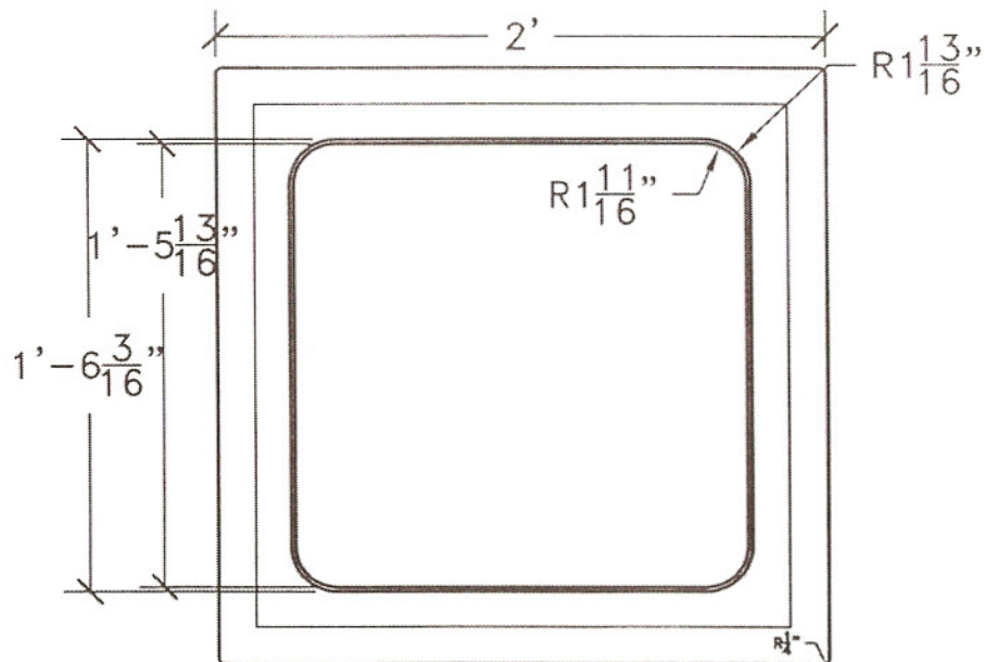
4 1 REFLECTED PLAN HINGED ACCESS PANEL AP18 N/A SCALE: NTS
