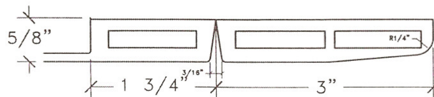
1 1 DETAIL HINGED ACCESS PANEL N/A AP18 SCALE: FULL
