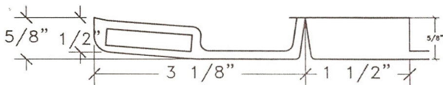
5 1 DETAIL HINGED ACCESS PANEL N/A AP18 SCALE: FULL
